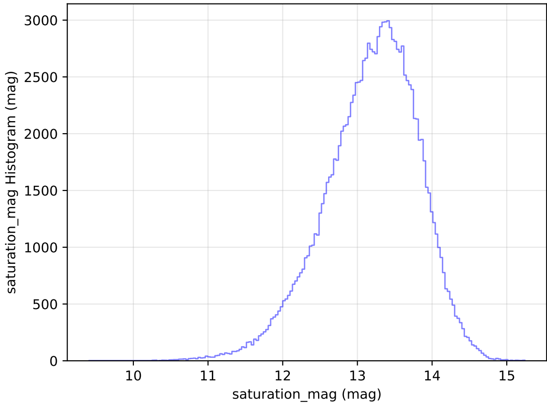
internal_u_expt38_nscale1.1v3.4_10yrs WFD u band: saturation_mag Histogram
