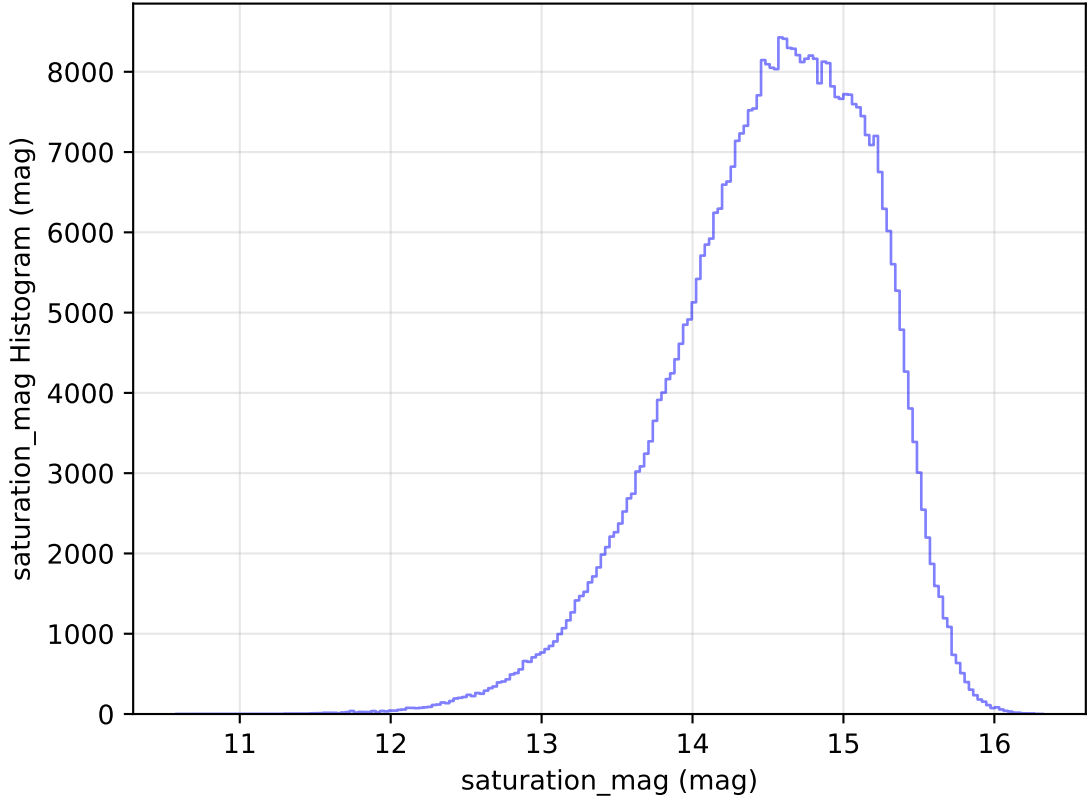
internal_u_expt38_nscale1.1v3.4_10yrs WFD r band: saturation_mag Histogram
