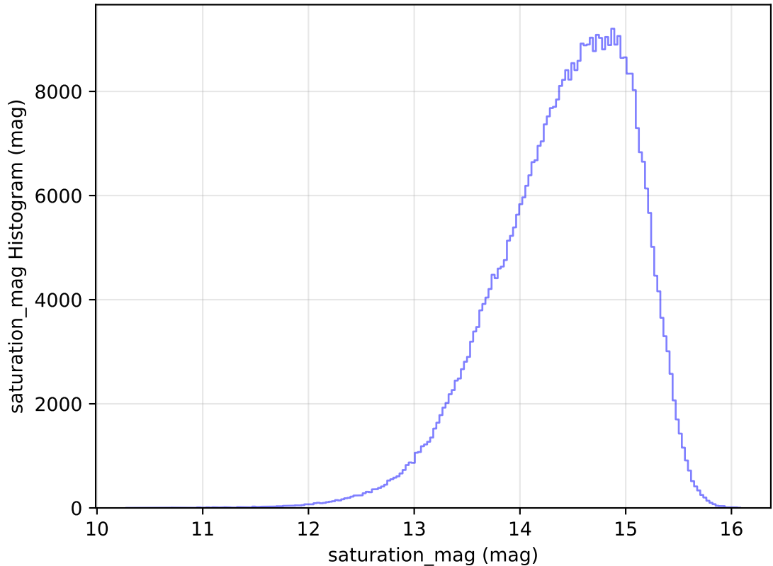
internal_u_expt38_nscale1.1v3.4_10yrs WFD i band: saturation_mag Histogram
