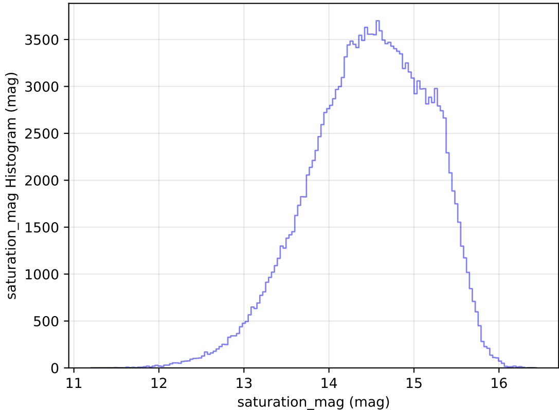
internal_u_expt38_nscale1.1v3.4_10yrs WFD g band: saturation_mag Histogram
