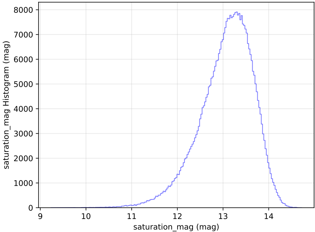
internal_u_expt38_nscale1.1v3.4_10yrs All sky y band: saturation_mag Histogram
