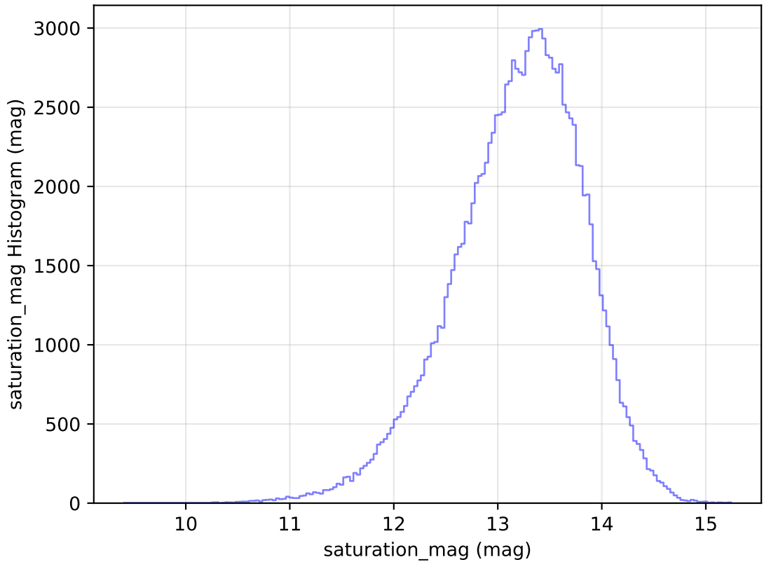
internal_u_expt38_nscale1.1v3.4_10yrs All sky u band: saturation_mag Histogram
