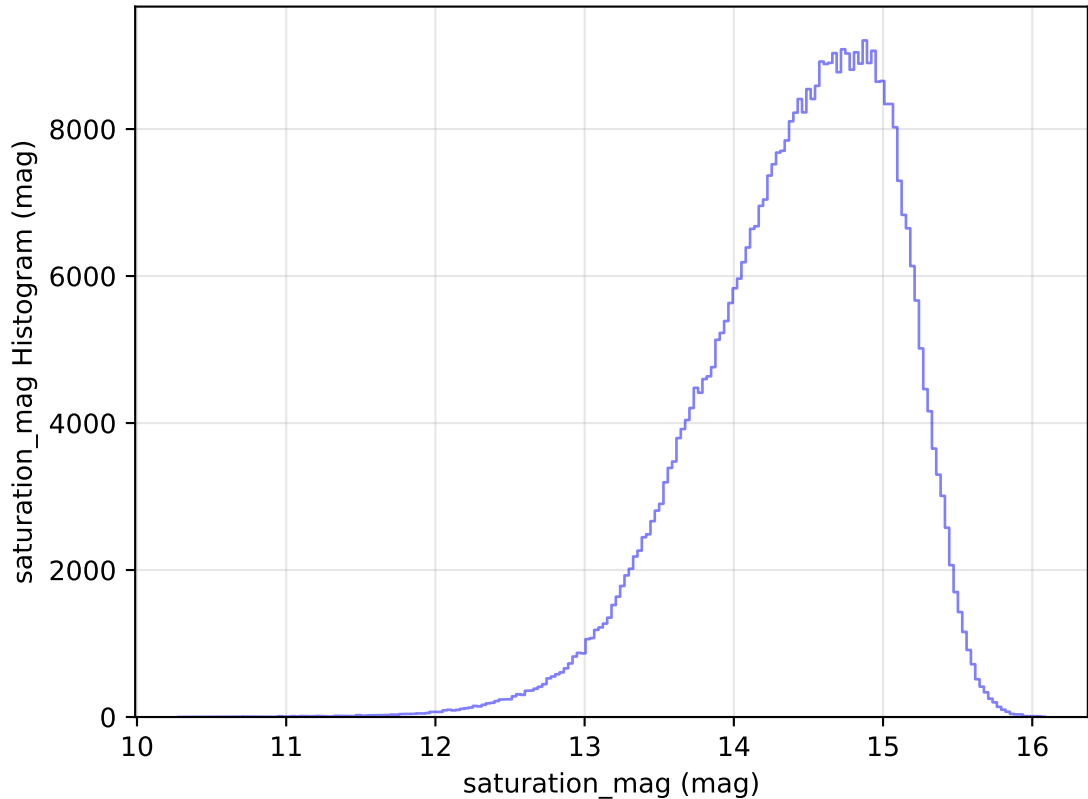
internal_u_expt38_nscale1.1v3.4_10yrs All sky i band: saturation_mag Histogram
