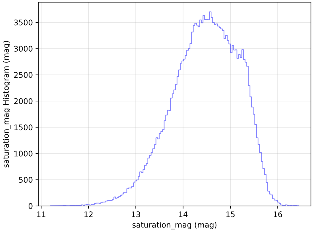
internal_u_expt38_nscale1.1v3.4_10yrs All sky g band: saturation_mag Histogram
