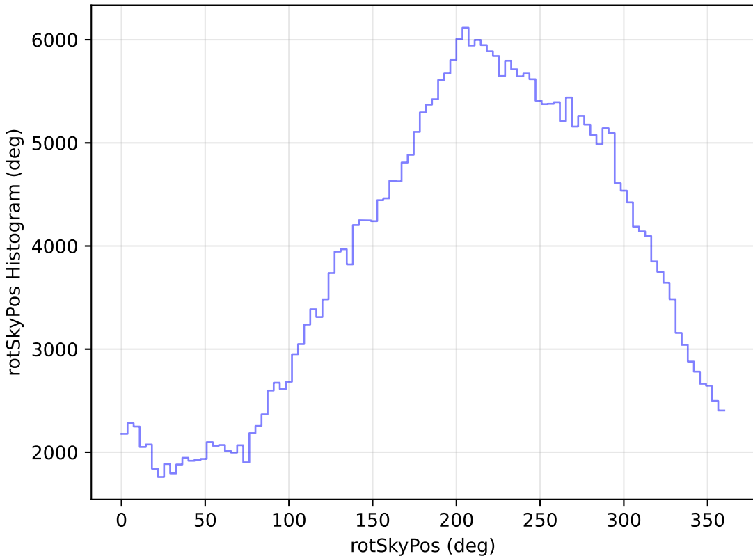
internal_u_expt38_nscale1.1v3.4_10yrs WFD y band: rotSkyPos Histogram
