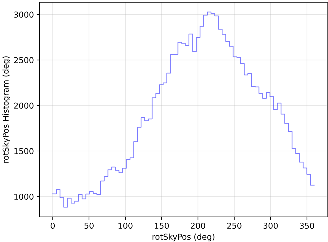
internal_u_expt38_nscale1.1v3.4_10yrs WFD u band: rotSkyPos Histogram
