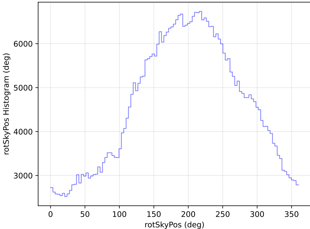
internal_u_expt38_nscale1.1v3.4_10yrs WFD r band: rotSkyPos Histogram
