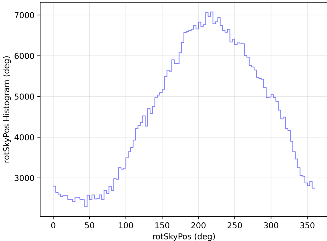
internal_u_expt38_nscale1.1v3.4_10yrs WFD i band: rotSkyPos Histogram
