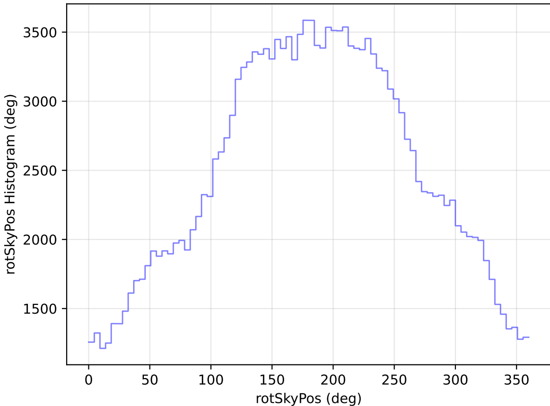
internal_u_expt38_nscale1.1v3.4_10yrs WFD g band: rotSkyPos Histogram
