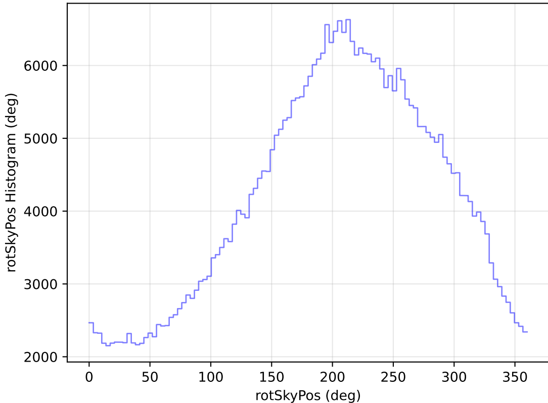
internal_u_expt38_nscale1.1v3.4_10yrs All sky z band: rotSkyPos Histogram
