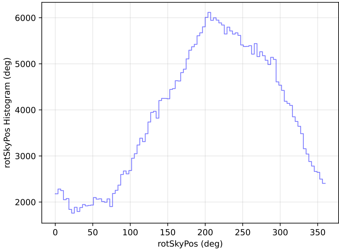
internal_u_expt38_nscale1.1v3.4_10yrs All sky y band: rotSkyPos Histogram
