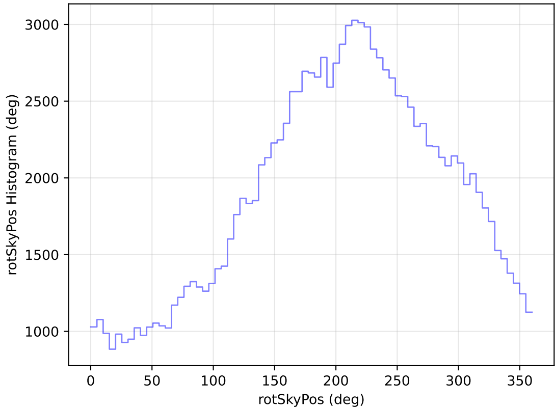
internal_u_expt38_nscale1.1v3.4_10yrs All sky u band: rotSkyPos Histogram
