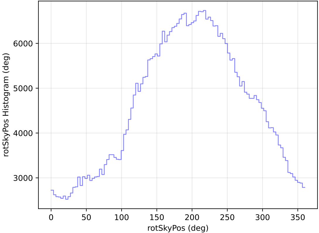
internal_u_expt38_nscale1.1v3.4_10yrs All sky r band: rotSkyPos Histogram
