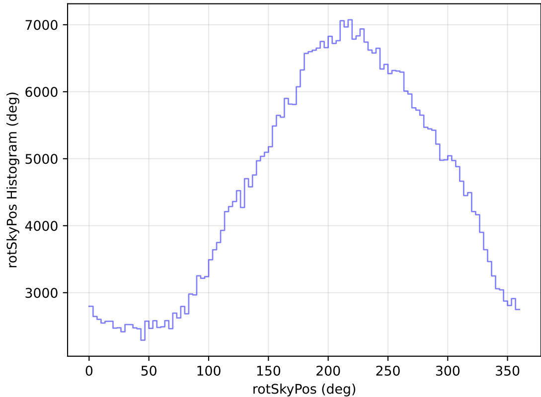
internal_u_expt38_nscale1.1v3.4_10yrs All sky i band: rotSkyPos Histogram
