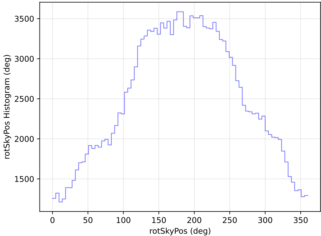
internal_u_expt38_nscale1.1v3.4_10yrs All sky g band: rotSkyPos Histogram
