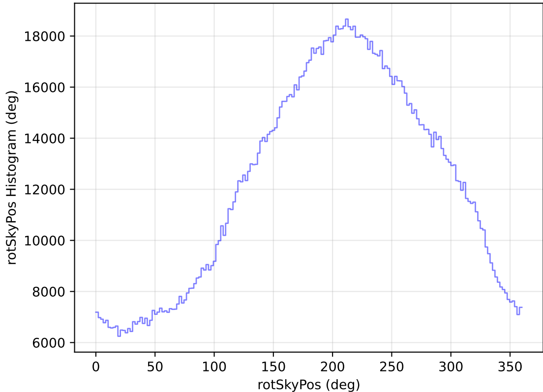
internal_u_expt38_nscale1.1v3.4_10yrs All sky all bands: rotSkyPos Histogram
