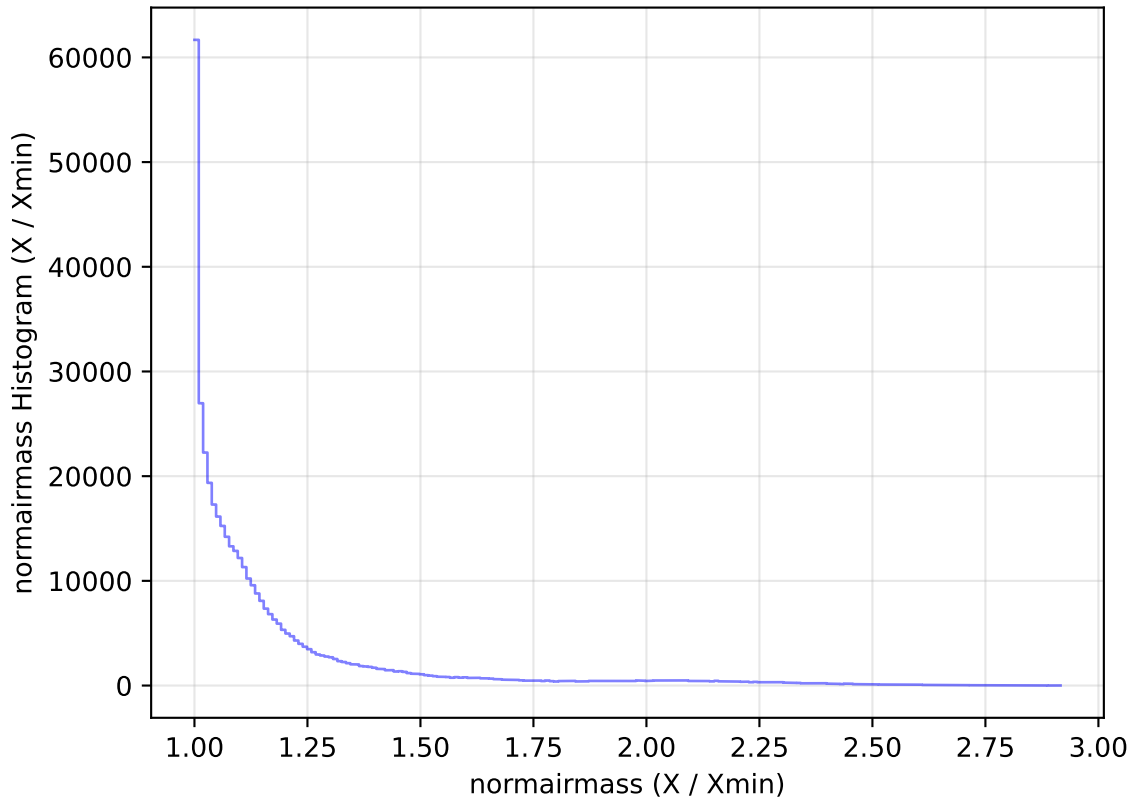
internal_u_expt38_nscale1.1v3.4_10yrs WFD z band: normairmass Histogram
