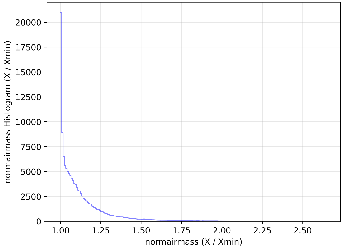
internal_u_expt38_nscale1.1v3.4_10yrs WFD u band: normairmass Histogram
