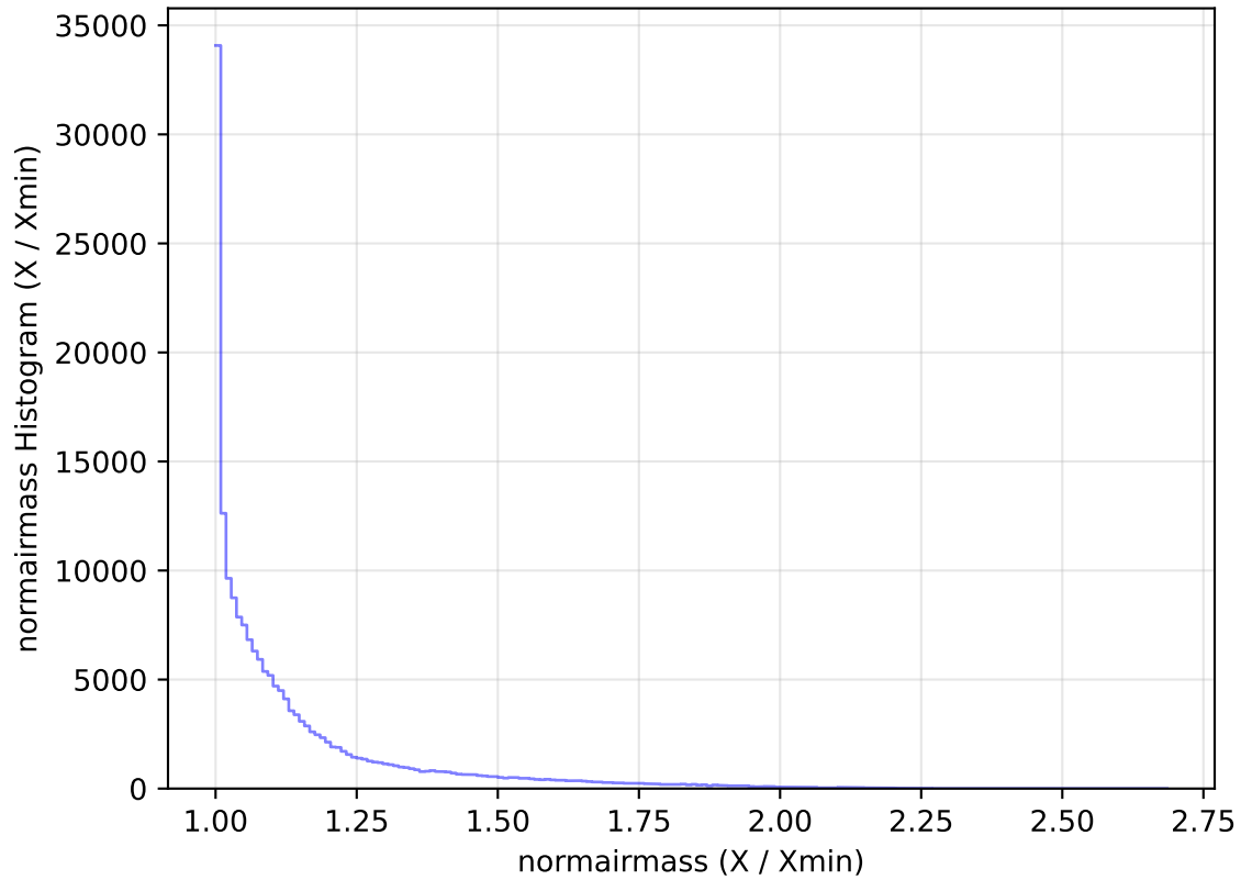
internal_u_expt38_nscale1.1v3.4_10yrs WFD g band: normairmass Histogram
