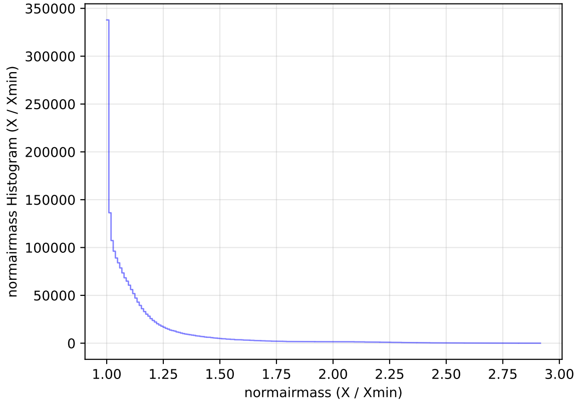
internal_u_expt38_nscale1.1v3.4_10yrs WFD all bands: normairmass Histogram
