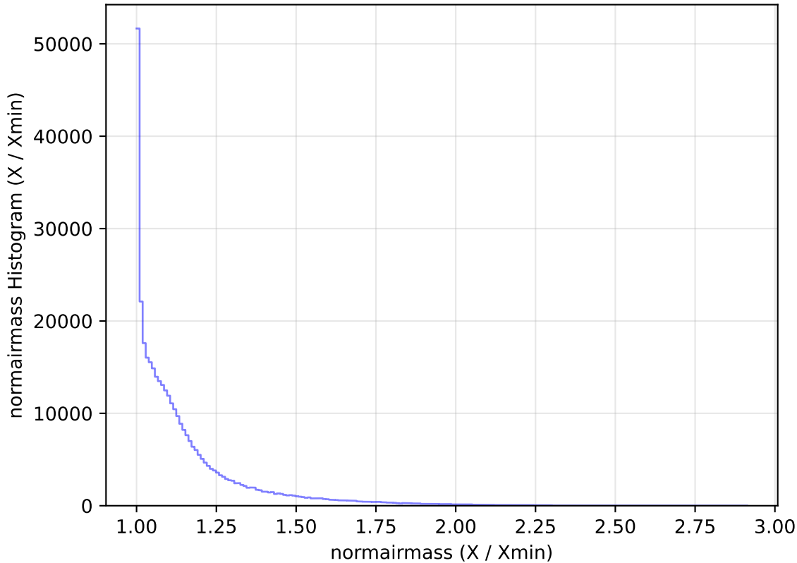
internal_u_expt38_nscale1.1v3.4_10yrs All sky y band: normairmass Histogram
