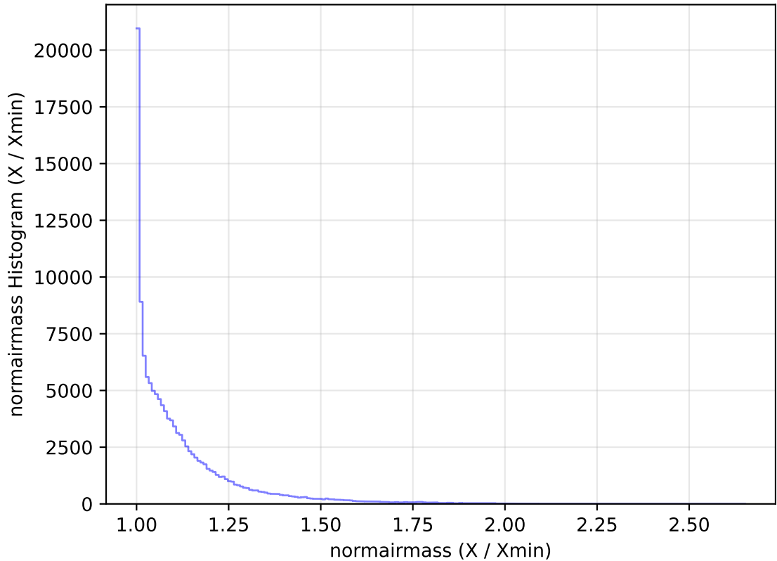
internal_u_expt38_nscale1.1v3.4_10yrs All sky u band: normairmass Histogram
