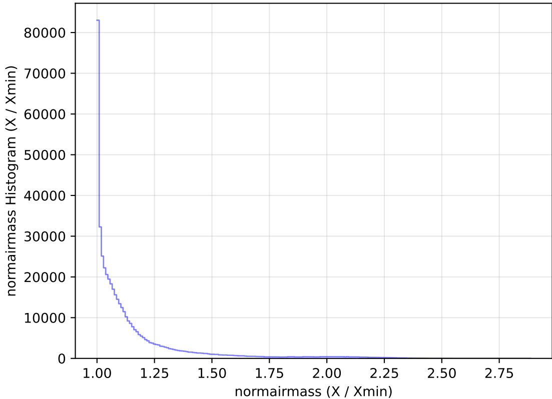
internal_u_expt38_nscale1.1v3.4_10yrs All sky r band: normairmass Histogram
