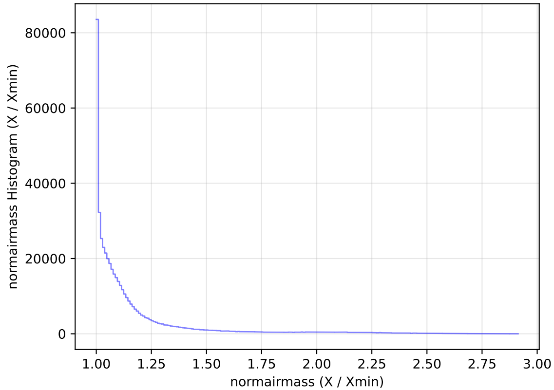
internal_u_expt38_nscale1.1v3.4_10yrs All sky i band: normairmass Histogram
