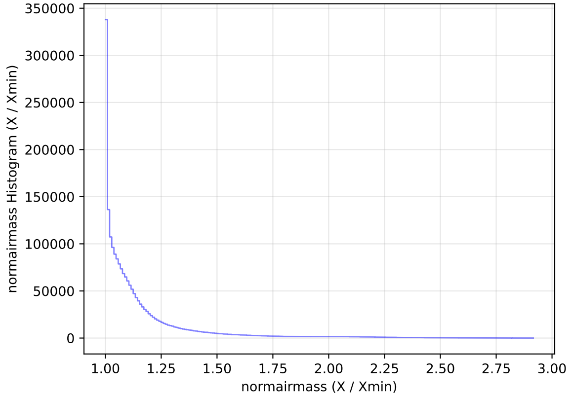
internal_u_expt38_nscale1.1v3.4_10yrs All sky all bands: normairmass Histogram
