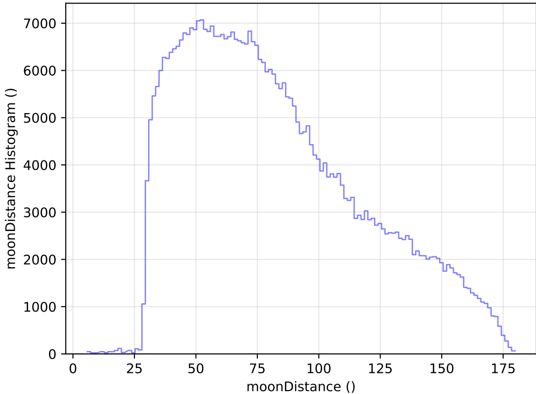
internal_u_expt38_nscale1.1v3.4_10yrs WFD z band: moonDistance Histogram
