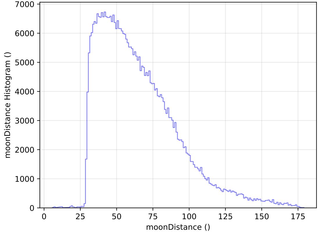
internal_u_expt38_nscale1.1v3.4_10yrs WFD y band: moonDistance Histogram
