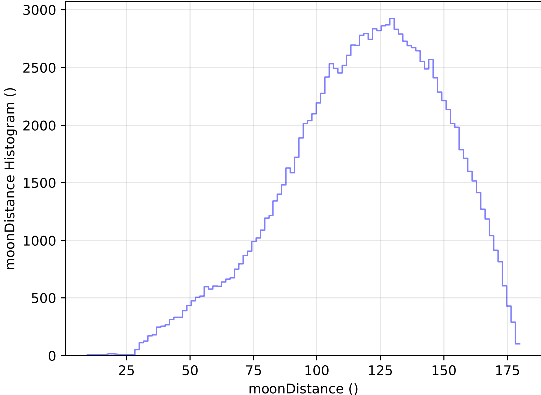
internal_u_expt38_nscale1.1v3.4_10yrs WFD u band: moonDistance Histogram
