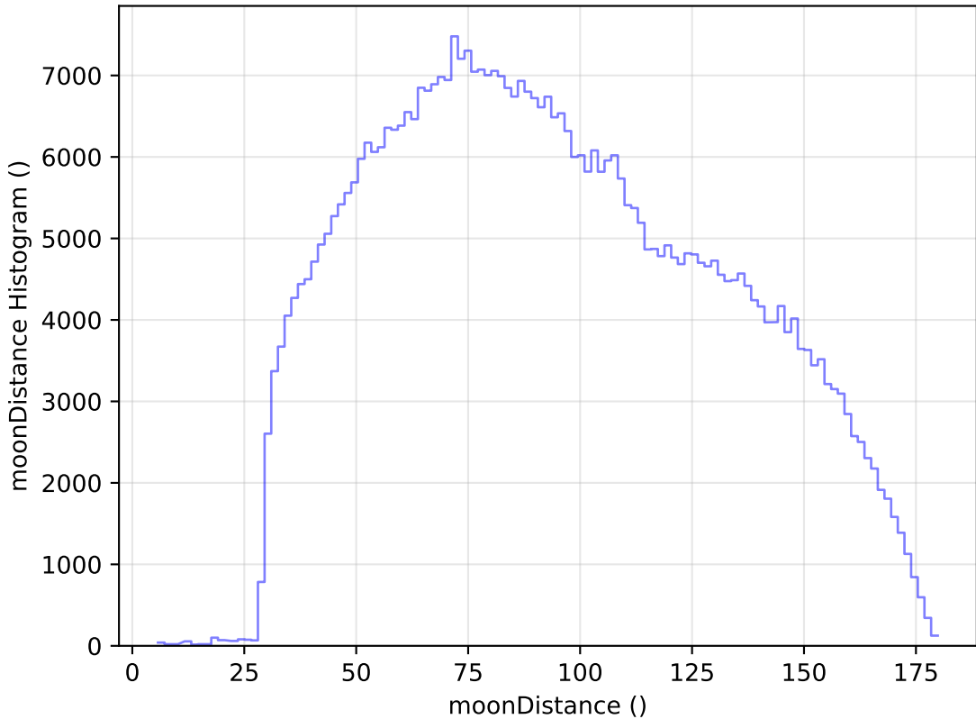
internal_u_expt38_nscale1.1v3.4_10yrs WFD i band: moonDistance Histogram
