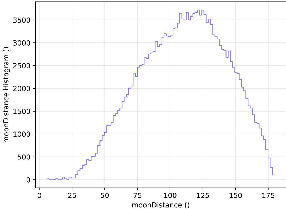
internal_u_expt38_nscale1.1v3.4_10yrs WFD g band: moonDistance Histogram
