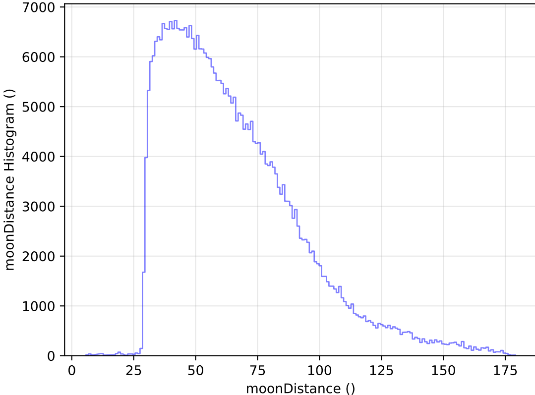
internal_u_expt38_nscale1.1v3.4_10yrs All sky y band: moonDistance Histogram
