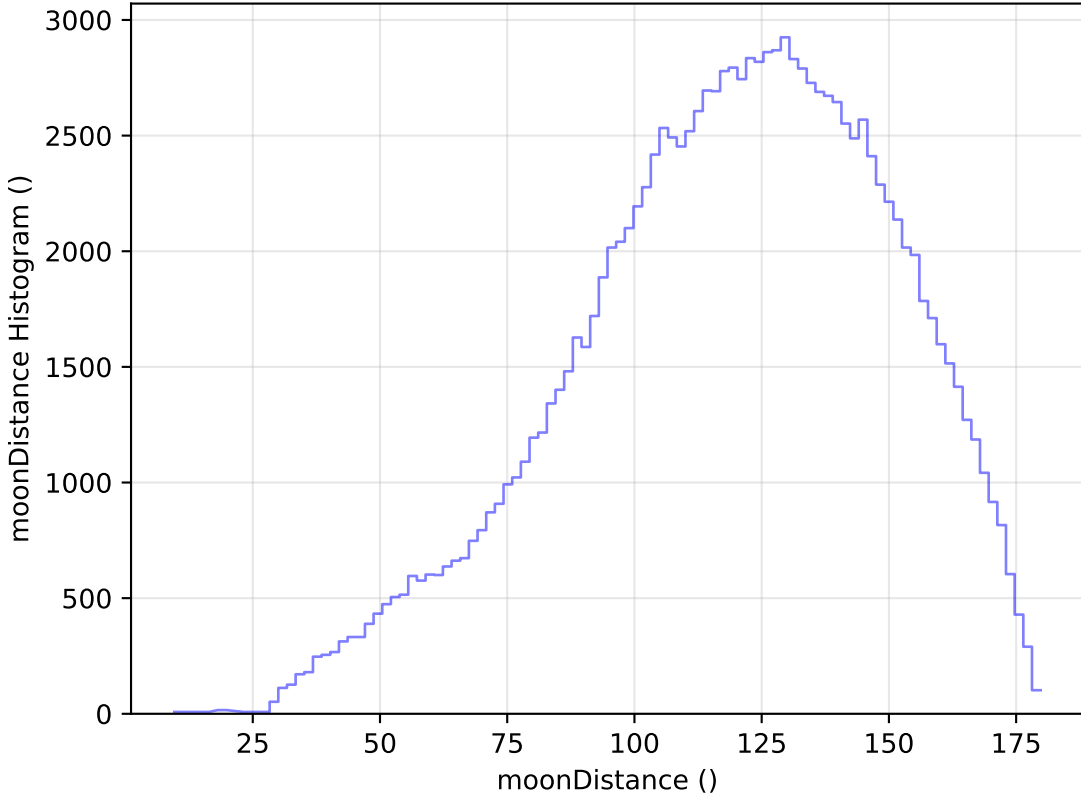
internal_u_expt38_nscale1.1v3.4_10yrs All sky u band: moonDistance Histogram
