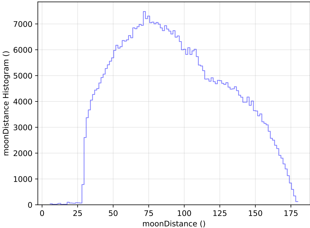
internal_u_expt38_nscale1.1v3.4_10yrs All sky i band: moonDistance Histogram
