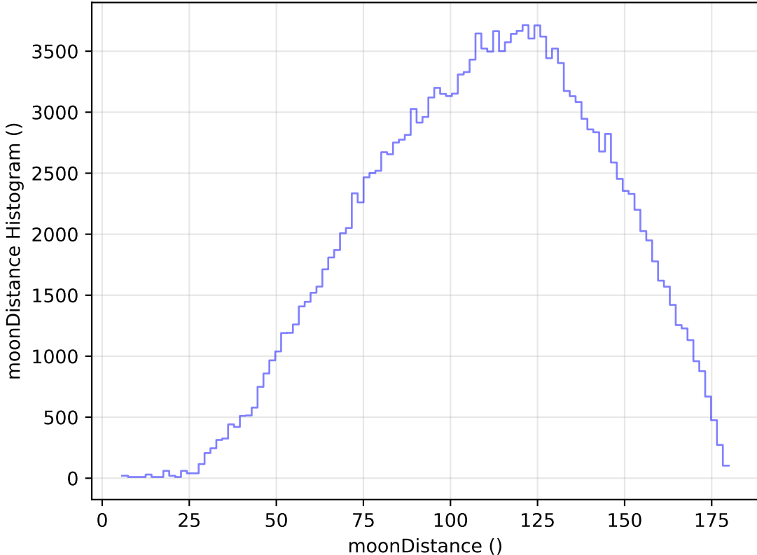
internal_u_expt38_nscale1.1v3.4_10yrs All sky g band: moonDistance Histogram
