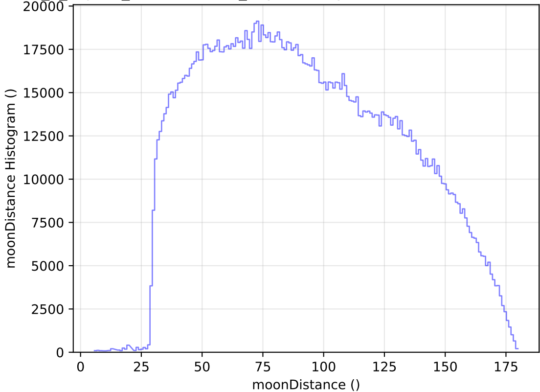
internal_u_expt38_nscale1.1v3.4_10yrs All sky all bands: moonDistance Histogram
