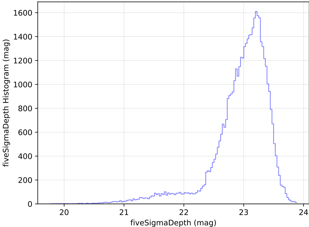
internal_u_expt38_nscale1.1v3.4_10yrs Yr 1 z band: fiveSigmaDepth Histogram
