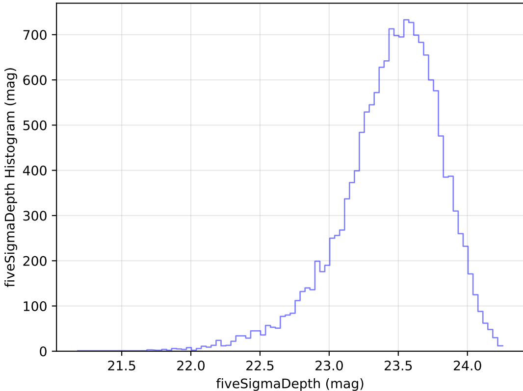
internal_u_expt38_nscale1.1v3.4_10yrs Yr 1 u band: fiveSigmaDepth Histogram
