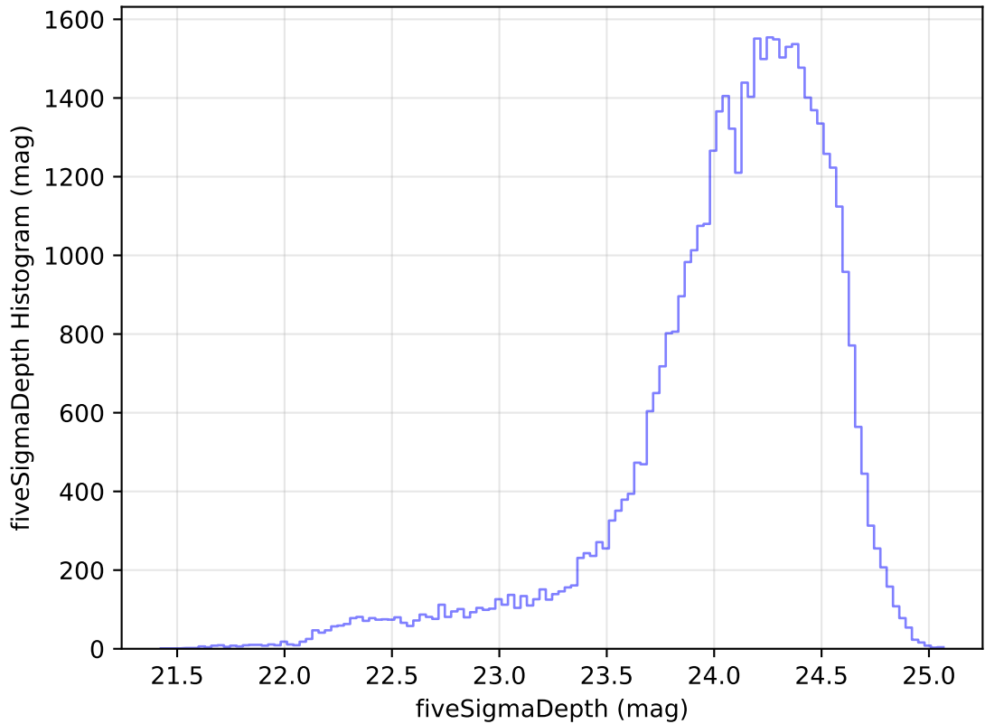
internal_u_expt38_nscale1.1v3.4_10yrs Yr 1 r band: fiveSigmaDepth Histogram
