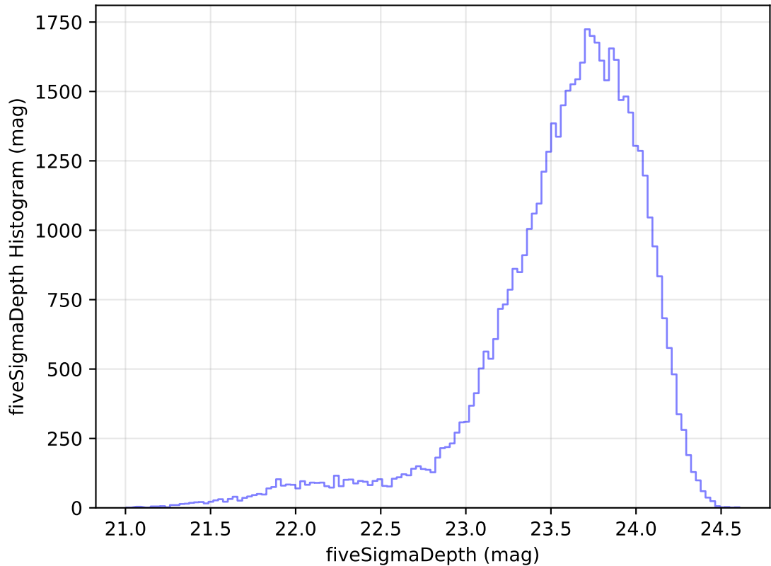
internal_u_expt38_nscale1.1v3.4_10yrs Yr 1 i band: fiveSigmaDepth Histogram
