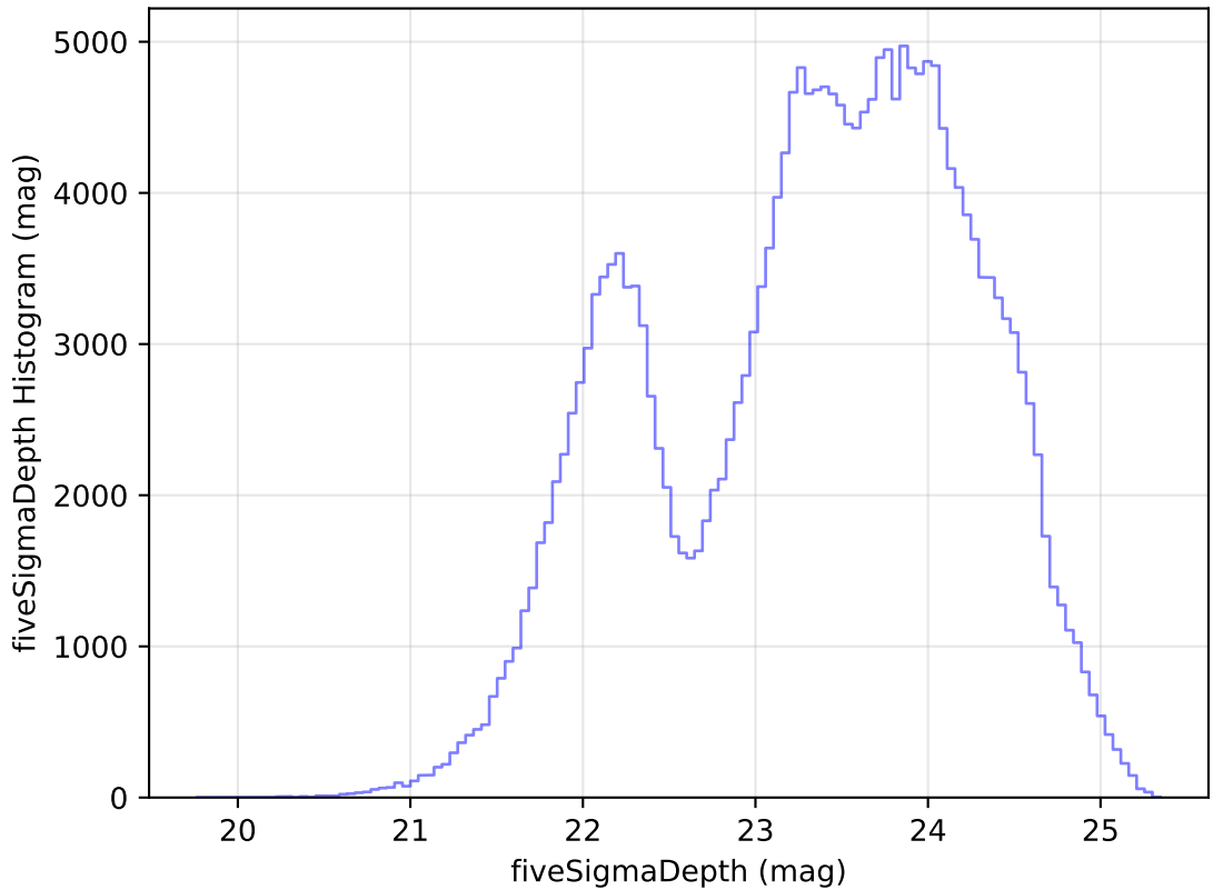
internal_u_expt38_nscale1.1v3.4_10yrs Yr 1 all bands: fiveSigmaDepth Histogram
