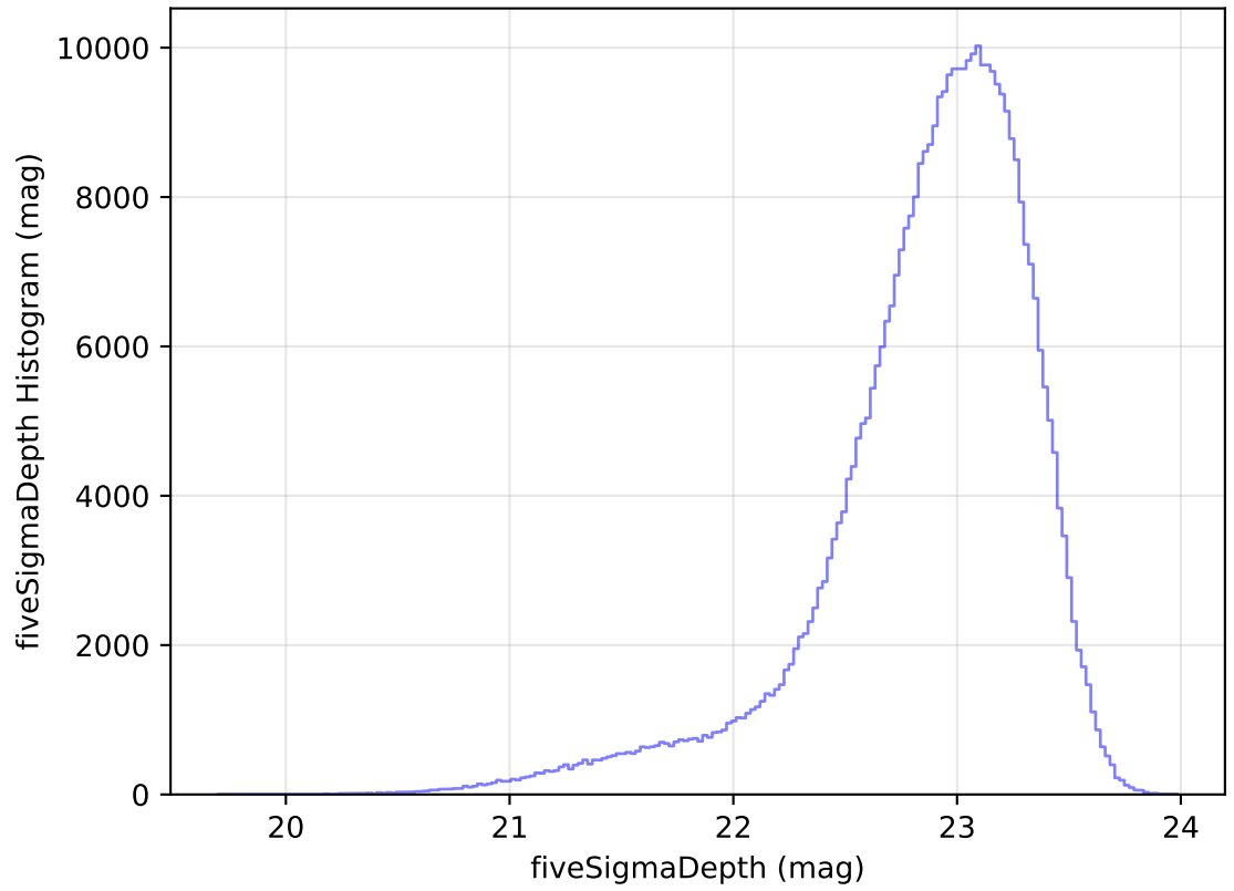
internal_u_expt38_nscale1.1v3.4_10yrs WFD z band: fiveSigmaDepth Histogram
