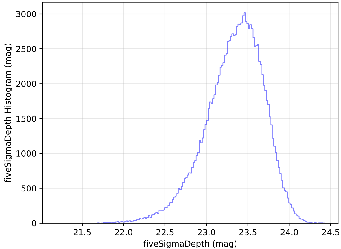
internal_u_expt38_nscale1.1v3.4_10yrs WFD u band: fiveSigmaDepth Histogram
