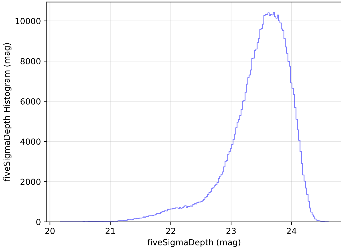
internal_u_expt38_nscale1.1v3.4_10yrs WFD i band: fiveSigmaDepth Histogram
