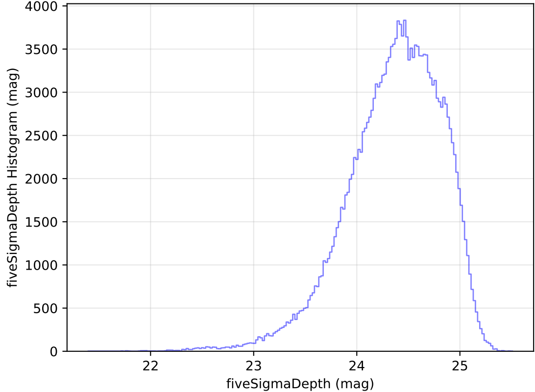
internal_u_expt38_nscale1.1v3.4_10yrs WFD g band: fiveSigmaDepth Histogram
