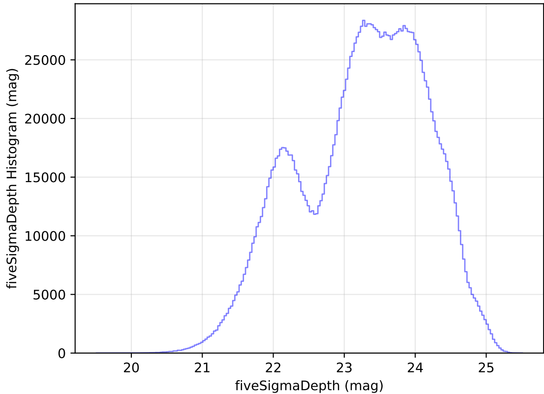
internal_u_expt38_nscale1.1v3.4_10yrs WFD all bands: fiveSigmaDepth Histogram
