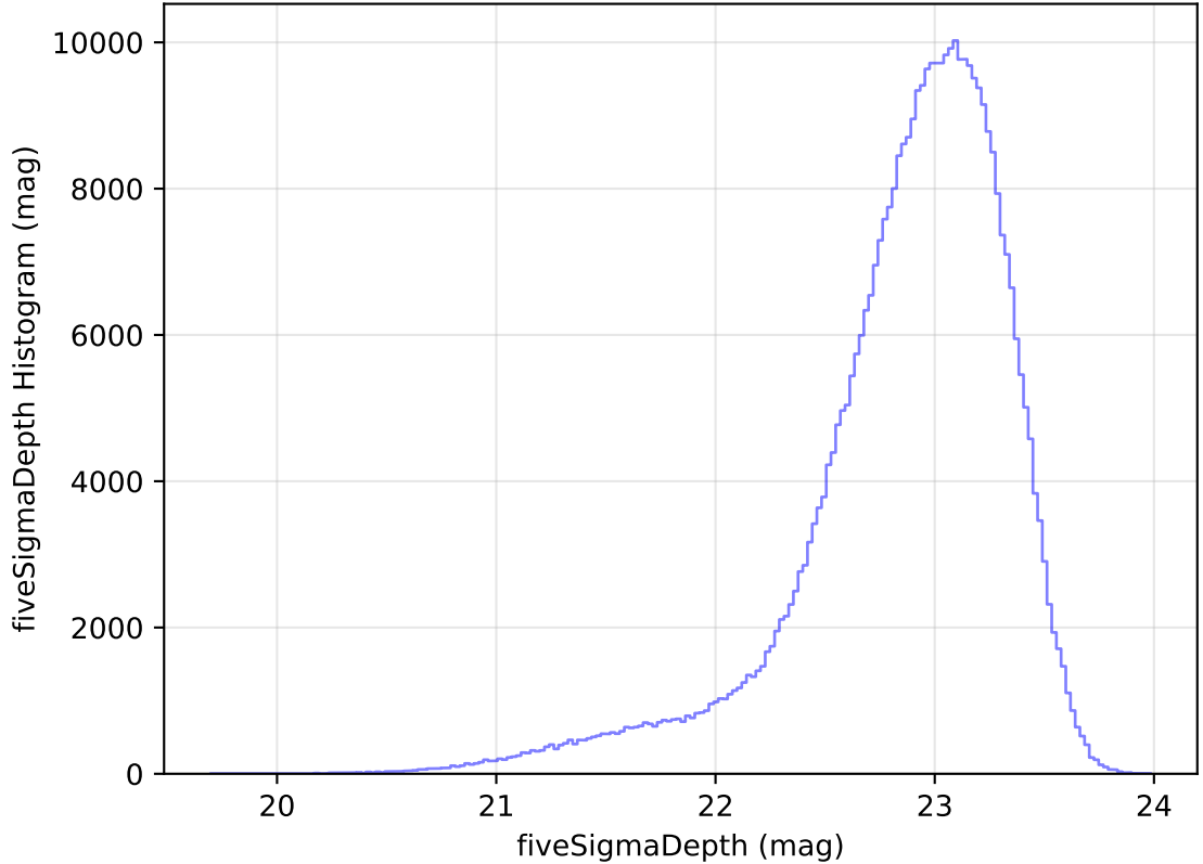
internal_u_expt38_nscale1.1v3.4_10yrs All sky z band: fiveSigmaDepth Histogram
